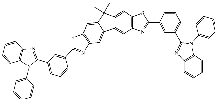
Compound 5
