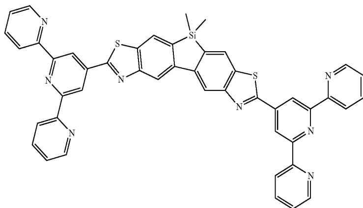
Compound 26
