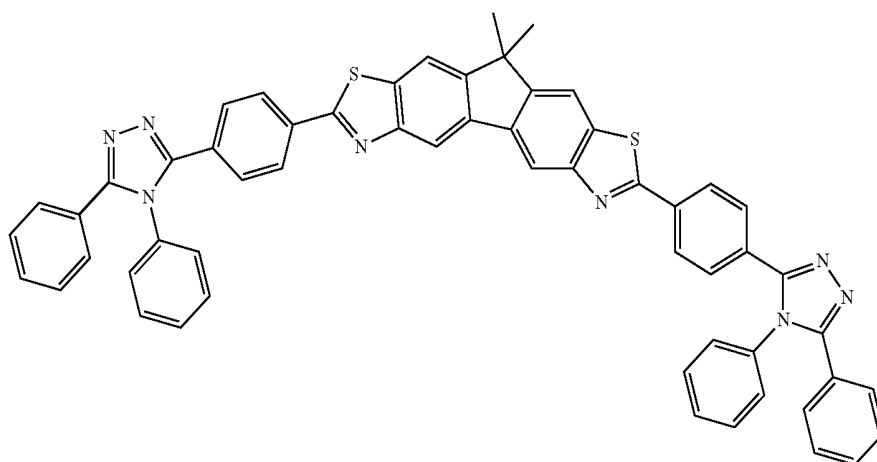
Compound 10
