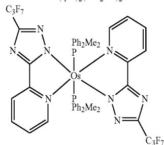
OS(hptz) 2 (PPhMe 2 ) 2
