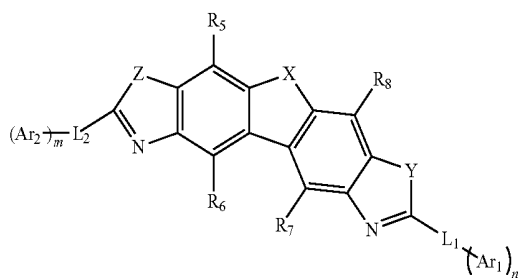
Formula 1
