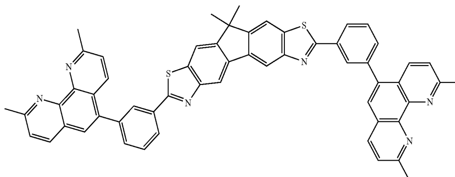
Compound 4
