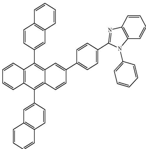
BAiq
