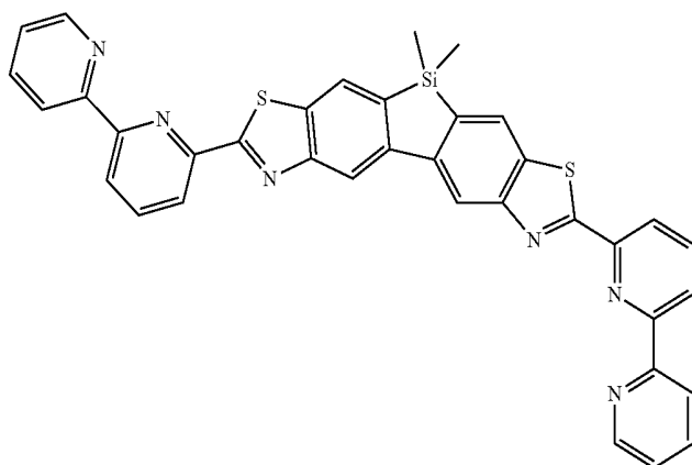
Compound 23
