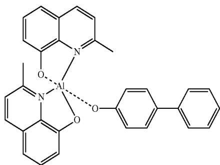
BAiq
