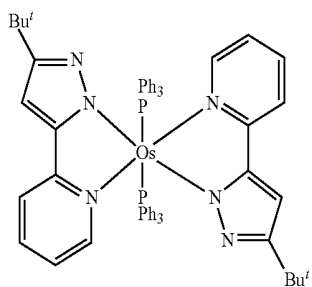
OS(bppz) 2 (PPh 2 Me) 2
